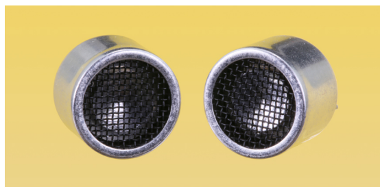
Figure 5-5 These components, listed as the “40TR12B-R ultrasonic sensor kit” by the online supplier Jameco, could form the basis of a DIY ultrasonic proximity sensor.
