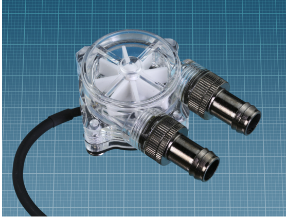
Figure 16-1 A low-cost, simple paddlewheel sensor designed for rates of 0.5 to 15 liters per minute. The background grid is in millimeters.
